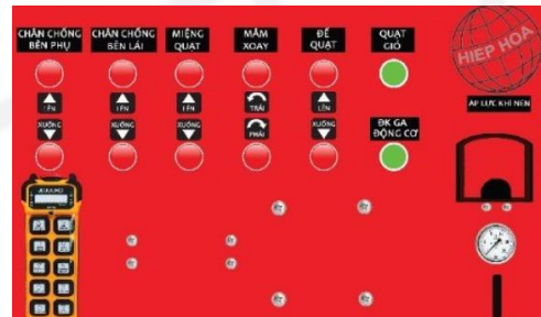
ELECTRIC REMOTE CONTROL SYSTEM Electric control with direct button and remote wirelessly. Control all working function of fan and engine.
